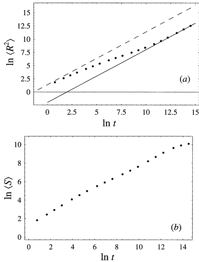
Figure 6. Average values for (a) walker displacement-squared R(t)^2 and (b) number S(t) of visited sites for walks over the indicated time intervals t through the composite shown in figure 5 (labyrinthine microstructure) with phase conductivity ratio \sigma_B/\sigma_A = 10^{-3} . The solid line in (a) is a fit to the data points in the Gaussian regime, while the dashed line indicates the walker behaviour in a single-phase material.
